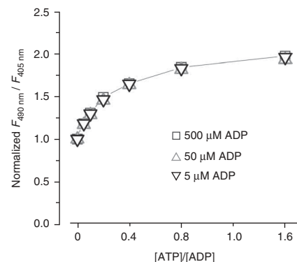
Figure 2 | The QV5 construct reports the ATP:ADP ratio. The QV5 construct fluorescence response to ATP application in the presence of 5 \mu\text{M} , 50 \mu\text{M} and 500 \mu\text{M} ADP showed a half-maximal response at 1 \mu\text{M} , 10 \mu\text{M} and 100 \mu\text{M} ATP, respectively, corresponding to a half-maximal response when [ATP]/[ADP] = \sim 0.2 .
